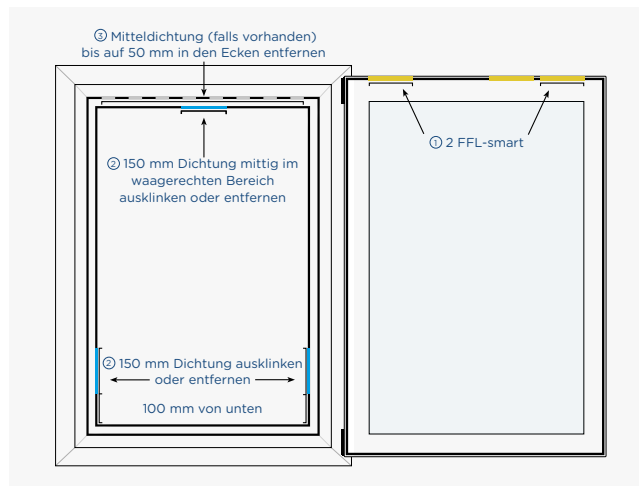
3 FFL-smart Standard
