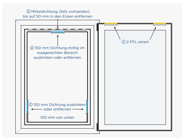
2 FFL-smart Standard
